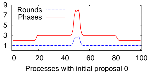
Processes with initial proposal 0 Figure 2: Complexity of Algorithm 3
