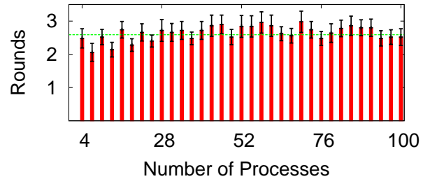
Figure 1: Round complexity of Algorithm 1 in a LAN same proposal and reach the agreement in one round. With the speculative algorithm, our previous analysis shows that when (from Lemma 2) \frac{n}{2} + k_2n processes (with k_2 > \frac{1}{4} ) propose the same value, then the agreement is achieved just in 2 phases.
