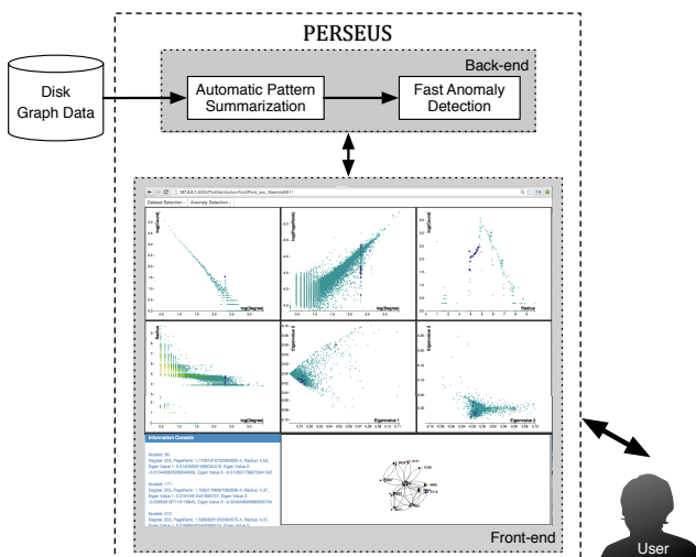
Figure 1: Perseus: system overview. The input graph is automatically processed to summarize graph statistics which are used for offline anomaly detection and visualization. The front-end visualization module, combines the graph properties and anomalies in six linked plots and a dynamic egonet.
