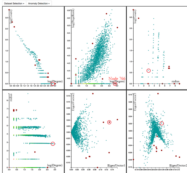
Figure 5: System-guided anomaly detection: The system flags node 766 as anomalous. Its corresponding points are highlighted in red circles.
