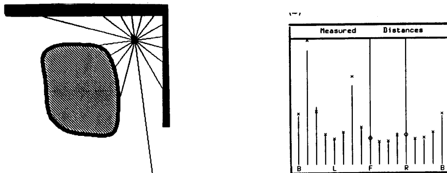
Figure 6: (a) NX in its environment; (b) NX's sensory image.
