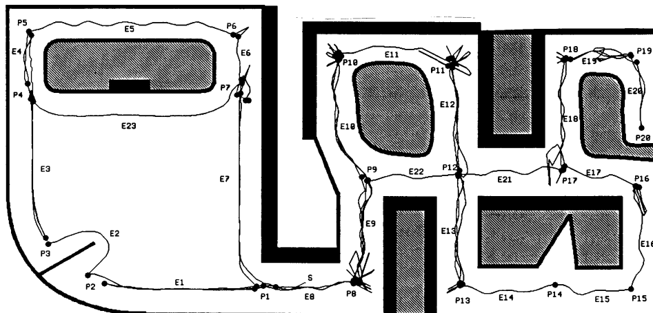
Figure 8: Exploration results with systematic and 10% random error
