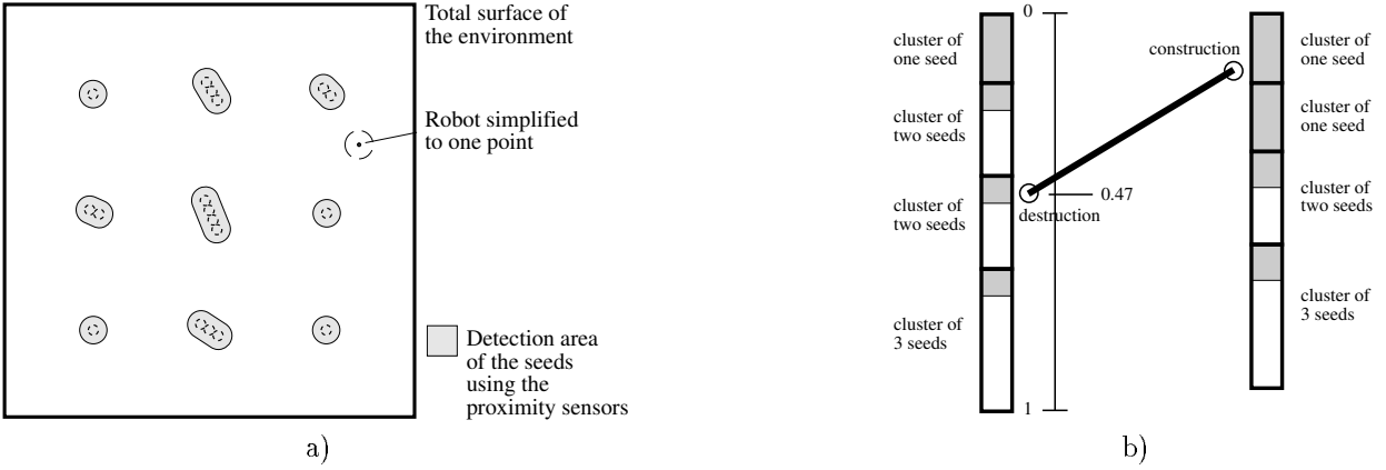
Figure 8: a) The first random process: the clusters are represented with their detection area scaled with the total surface of the environment; the probability that a robot encounters a cluster is proportional to the detection area of the cluster. b) The second random process: the robot can modify the size of the cluster, incrementing or decrementing it by 1 seed, only if the robot runs into the cluster from the positions described in fig. 5 or fig. 6. The two bars represent the whole set of clusters scattered at a given moment on the arena: if the random cursor (set on the left bar at 0.47) fails on a grey zone, the selected cluster will be decremented (left bar) or incremented (right bar) by 1 seed.
