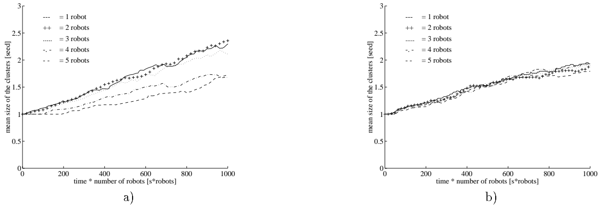
Figure 12: Mean fitness of the single teammate within a group composed by an increasing number of robots (1 to 5) on the arena of 80x80 cm and 20 seeds to gather. (a) Results of the experiments with the robots. (b) Results of the simulations.
