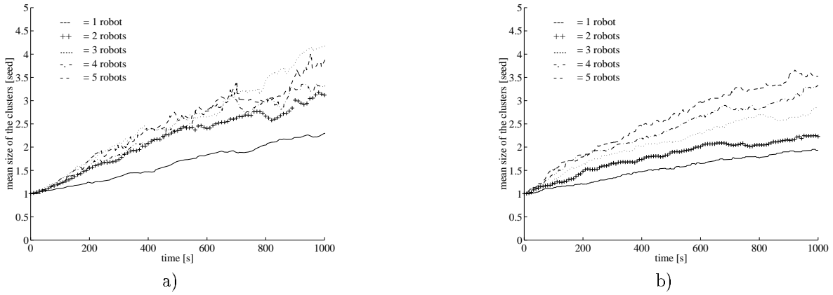
Figure 9: Fitness of the group with increasing number of robots (1 to 5) on the arena of 80x80 cm and 20 seeds to be gathered. (a) Results of the experiments with real robots. (b) Results of the simulations.
