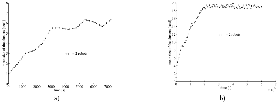
Figure 13: The evolution of cluster mean size during a) 2 hours with real robots and b) about 7 days in simulation (the time needed for this simulation is about 5 minutes on a SUN Sparc Station 20).
