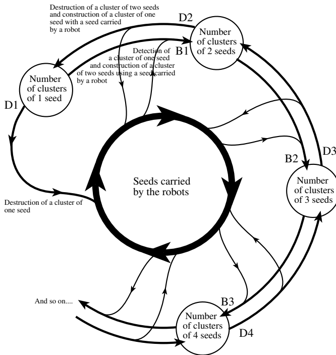
Figure 7: The dynamics of the clustering experiment represented as a probabilistic finite state machine.
