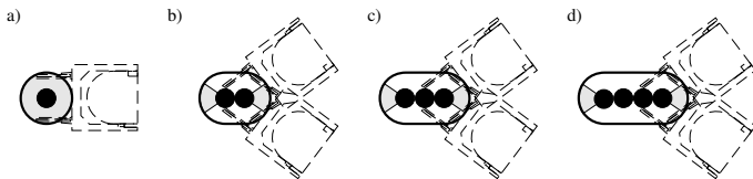
Figure 6: Geometrical representation of the destruction probability of a cluster: the robot, in order to decrement the size of the cluster of 1 seed has first to detect the cluster as in figure 5 and then grasp a seed. Due to the geometrical constraints of the gripper, the access perimeter for seed grasping is more limited than the detection perimeter. The resulting probability is therefore represented by the minimum of the two mentioned perimeters.
