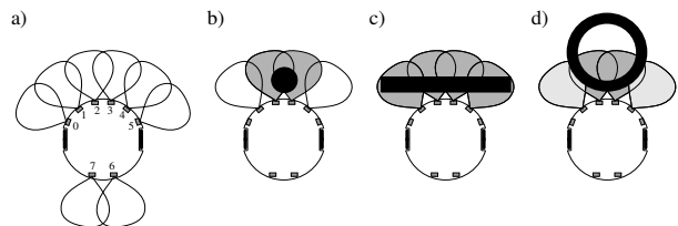
Figure 3: The detection lobes of the proximity sensors of the Khepera. A dark lobe means that the sensor is saturated, a light lobe means a low or zero activity.
