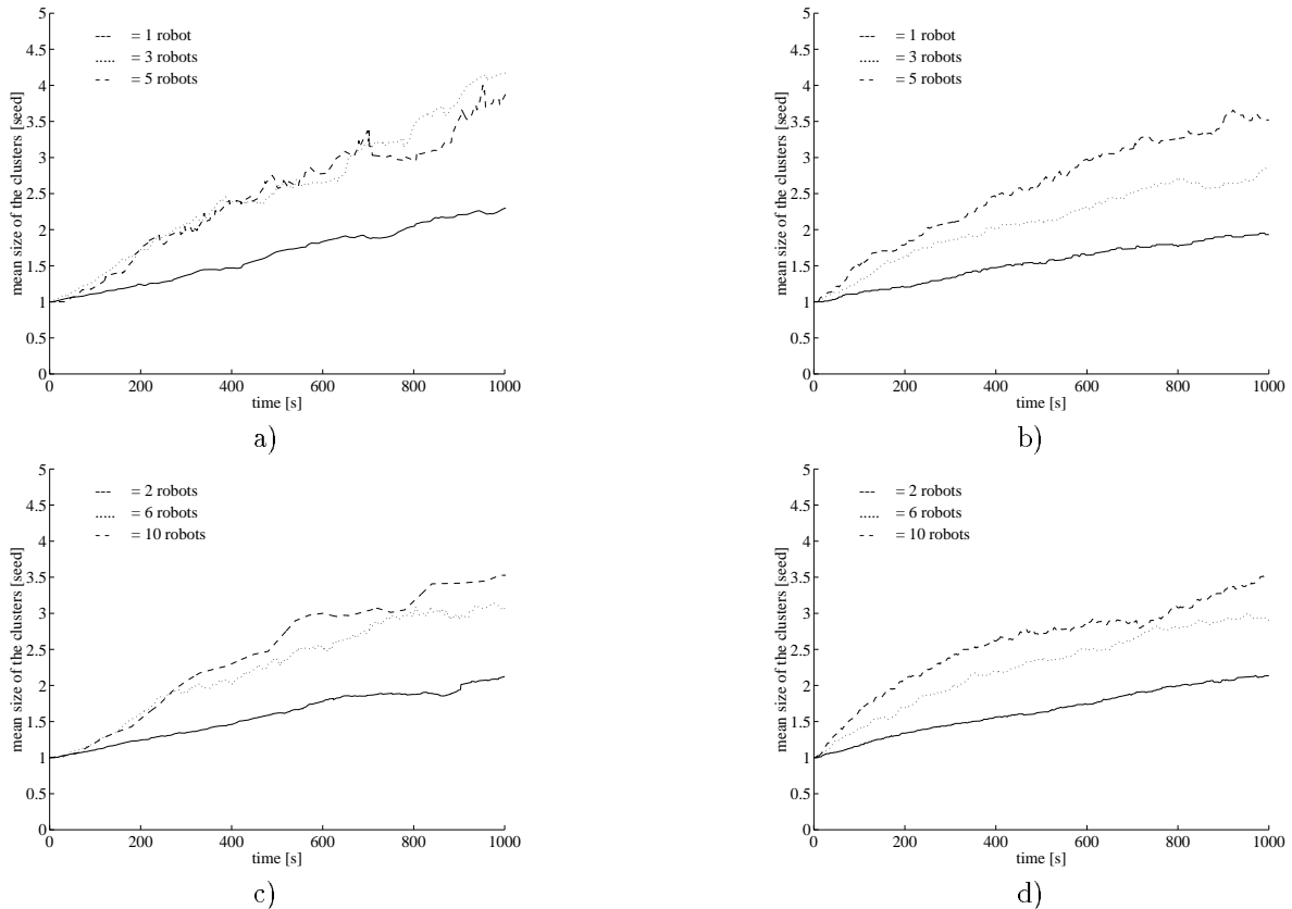
Figure 11: Fitness of the group with increasing number of robots (1,3 and 5) on the arena of 80x80 cm and 20 seeds to gather in a) and fitness of the group with the double of teammates (2,6 and 10), the double of seeds (40) and an arena two times bigger (113x113 cm) in c). The corresponding simulated fitnesses are depicted in figure b) and d).
