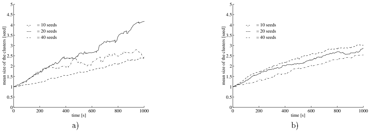
Figure 10: Fitness of the group with 3 robots and an increasing number of seeds (10, 20 and 40) on the arena of 80x80 cm. (a) Results of the experiment with the real robots. (b) Results of the simulations.
