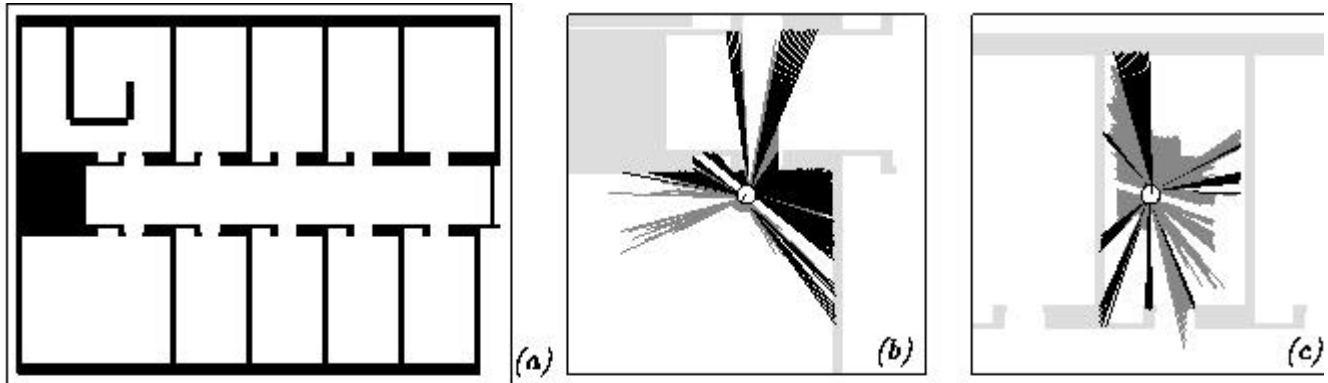
Fig. 15. (a) Outline of the office environment and (b,c) examples of filtered (grey) & incorporated (black) sensor readings using the distance filter.
