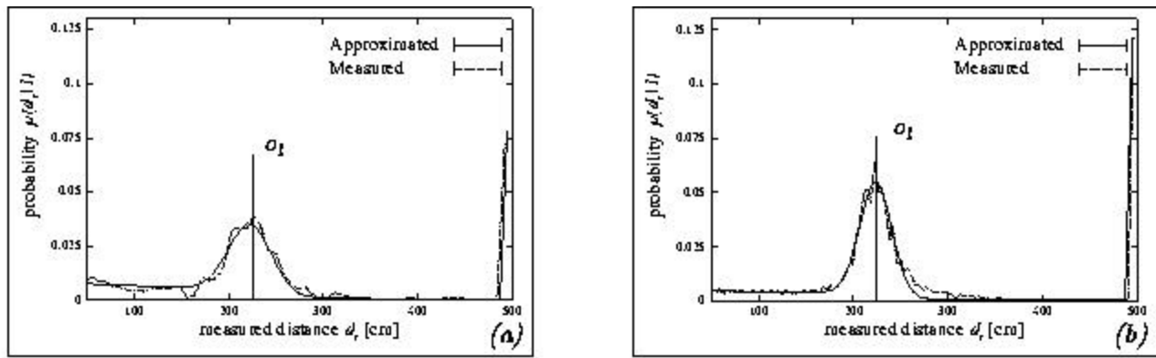
Fig. 5. Measured and approximated probabilities of (a) sonar and (b) laser measurement given the distance o_i to the closest obstacle along the sensing direction.
