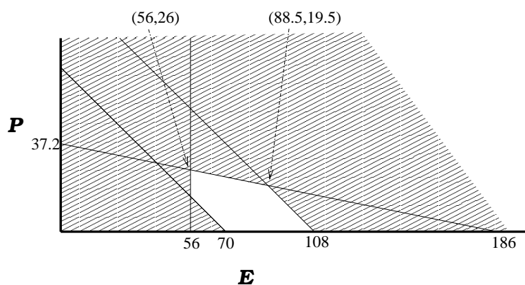
Figure 17.1: Feasible region for our time-planning problem. The constraints are: E \geq 56 ; P + E \geq 70 ; P \geq 0 ; S \geq 60 which means 168 - P - E \geq 60 or P + E \leq 108 ; and finally 2S - 3P + E \geq 150 which means 2(168 - P - E) - 3P + E \geq 150 or 5P + E \leq 186 .
