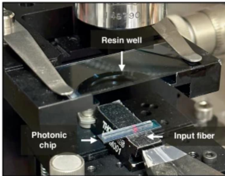
Experimental setup
