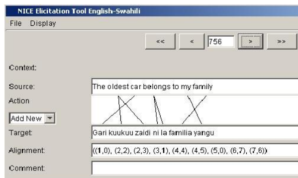
Figure 2: AVENUE elicitation interface
