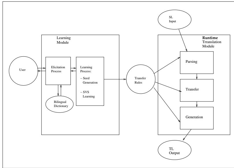
Figure 1: AVENUE system architecture
