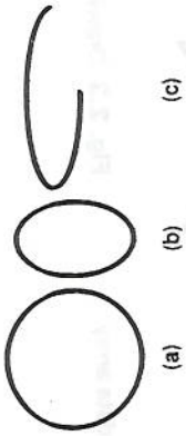
Fig. 2.5 Ellipse arcs.
