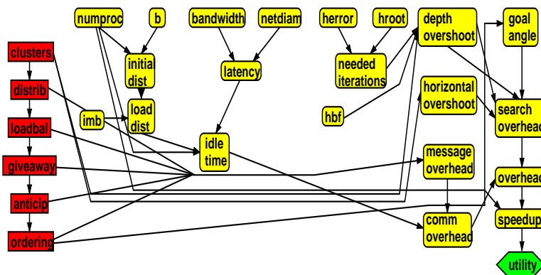
Figure 4: A model of the factors that influence speedup of parallel search algorithms.
