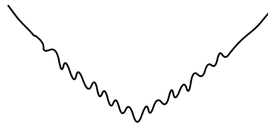
Figure 1: Intuitive picture of a “big valley” cost surface.
