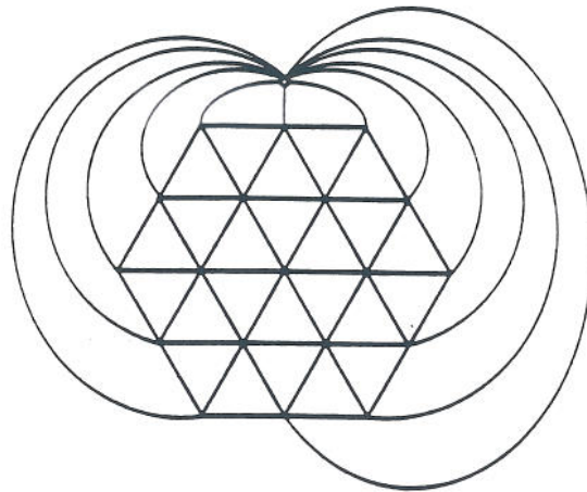
FIGURE 9. The boundary of the polyhedron used to show that t(n) \geq 2n - O(n^{1/2}) .
