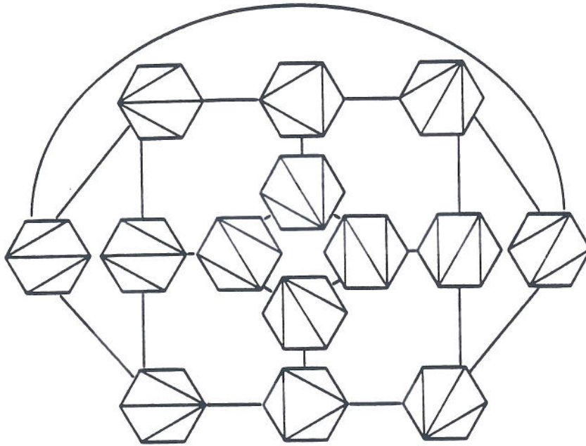
FIGURE 4. The rotation graph of a hexagon, RG(6) .
