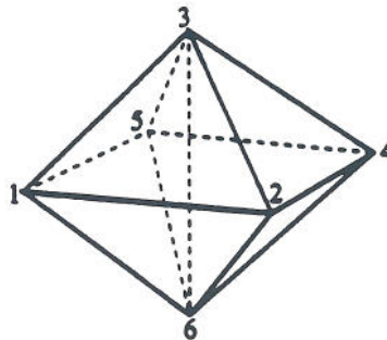
The four tetrahedra: 3 6 1 5, 3 6 2 1, 3 6 4 2, 3 6 5 4
