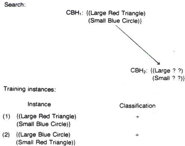
FIG. 3. Depth-first search example.
