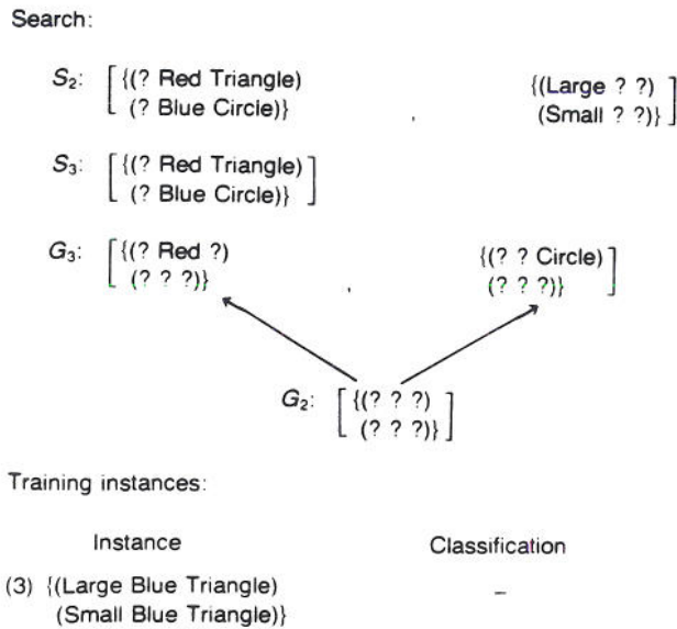
FIG. 10. Version space example (continued).
