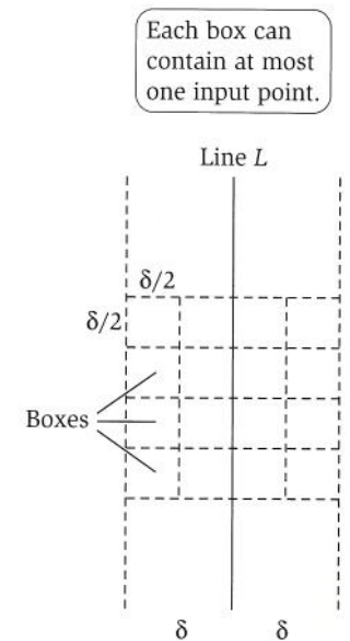
Figure 5.7 The portion of the plane close to the dividing line L , as analyzed in the proof of (5.10).
