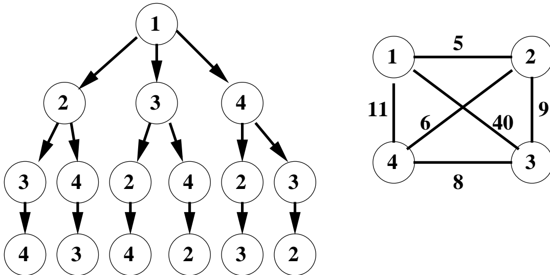
Figure 1: A TSP example
