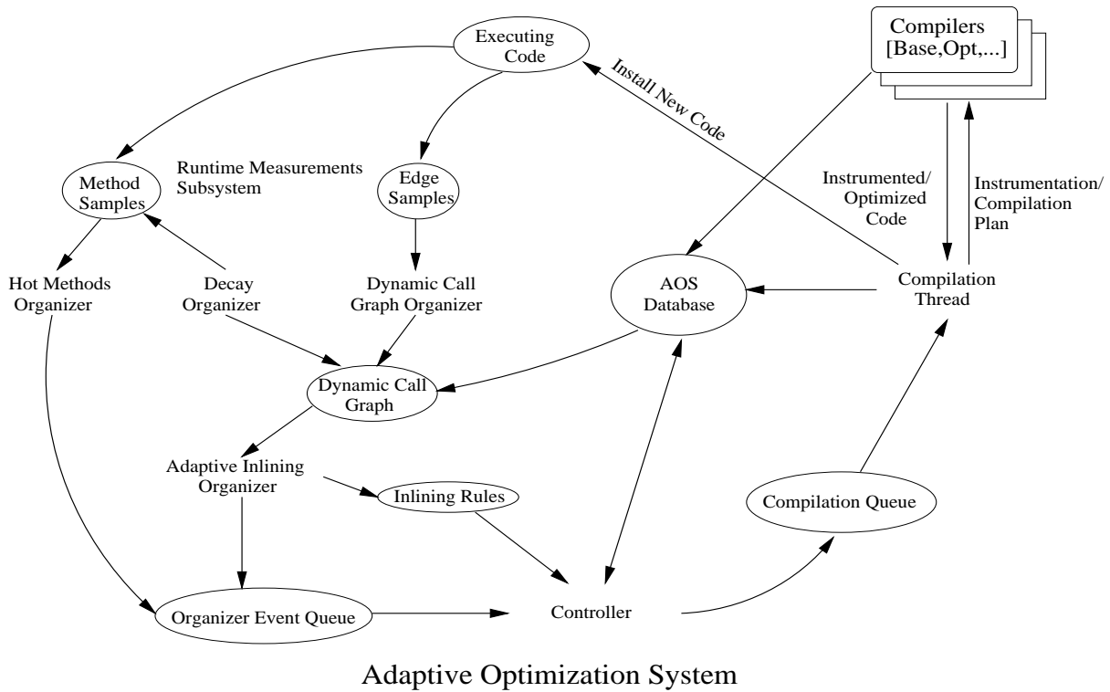
Figure 4: Implementation of feedback-directed inlining in the Jalapeño Adaptive Optimization System
