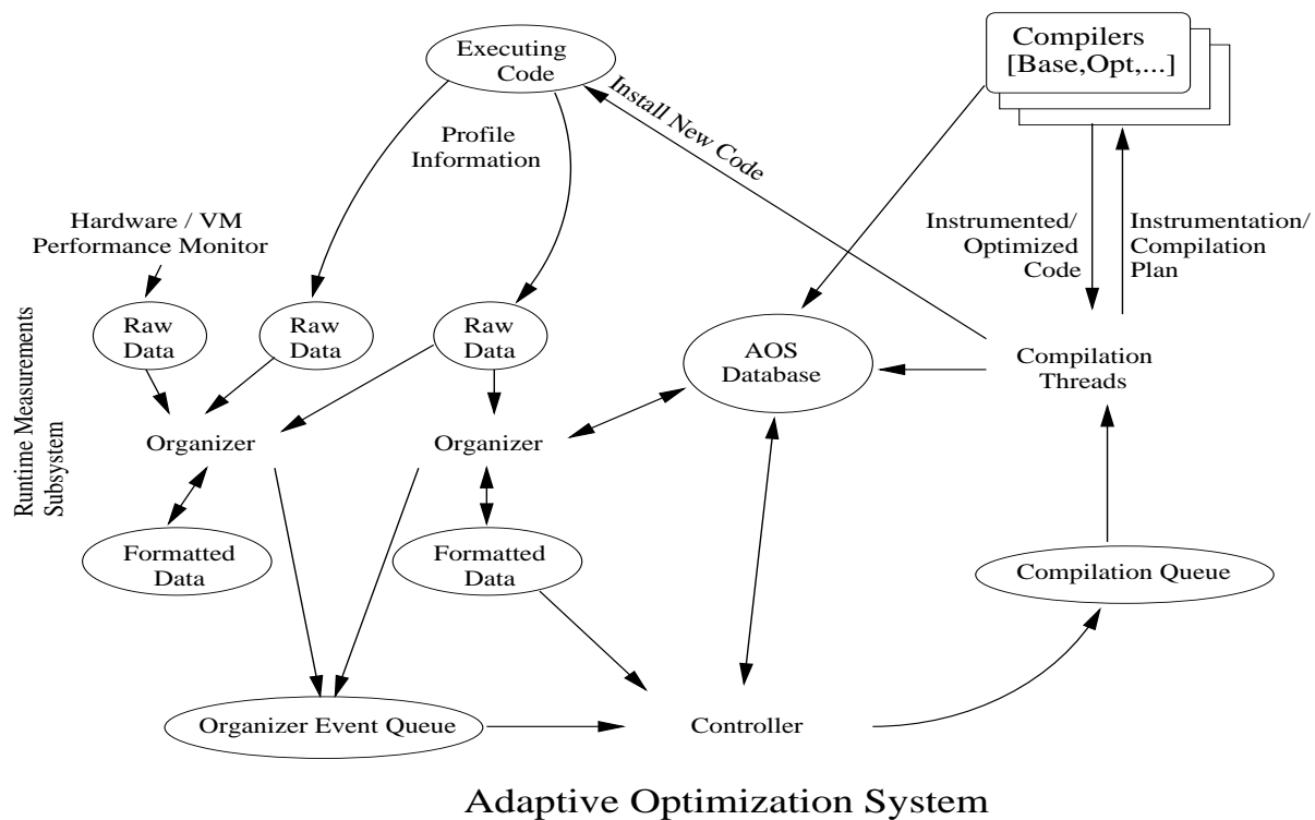
Figure 2: Architecture of the Jalapeño Adaptive Optimization System
