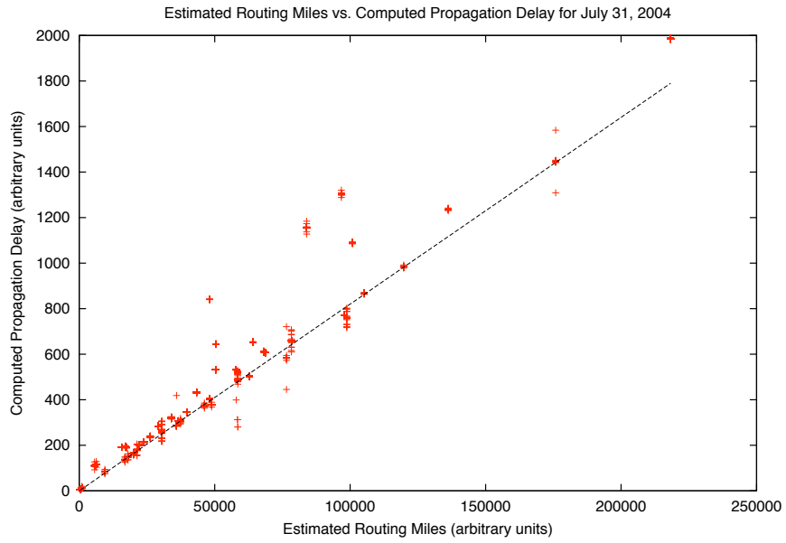
Figure 6.6: Plot of router miles versus computed propagation delay. The dashed line represents speed-of-light propagation.
