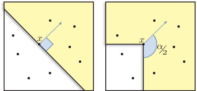
Figure 1: The \alpha -wedge depth counts points in wedges rather than halfspaces.
