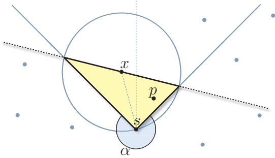
Figure 3: The triangle is H^- \cap W' and is completely contained in the ball centered at x .
