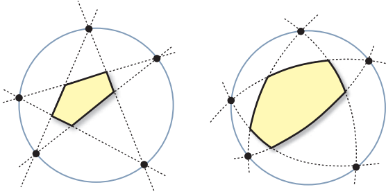
Figure 2: On the left, the center region for \alpha = \pi is the set of all centerpoints. On the right, the center region for \alpha > \pi replaces lines with circular arcs, expanding the set of centerpoints.
