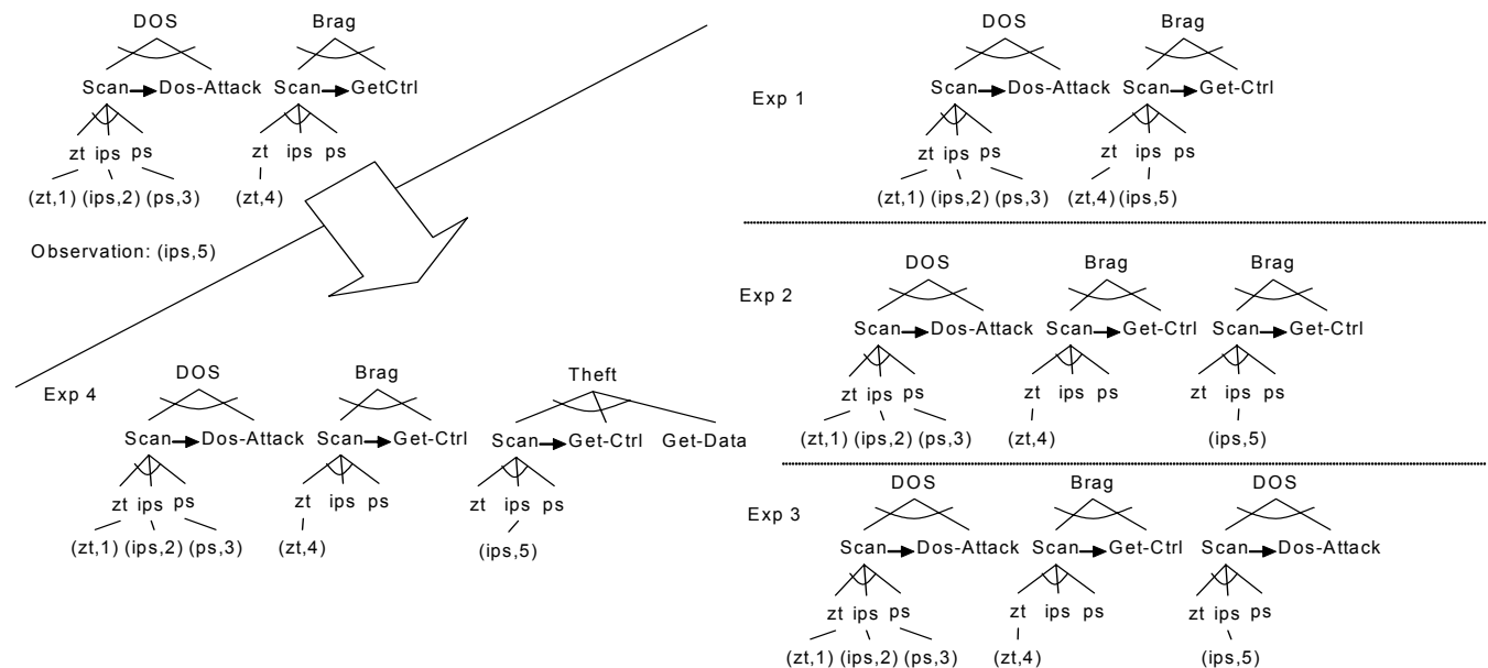
Figure 5: Upper Left: One of the explanations that explains an observation of the first unordered leaders. Lower Right: The four explanations required to explain the observation of the second unordered leader for the three root goals DOS, Brag, and Theft
