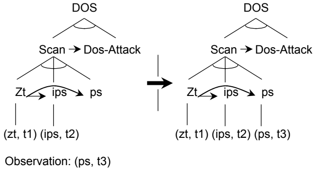
Figure 3: Left: an observation and explanation pair with a single point of attachment. Right: resulting explanation.
