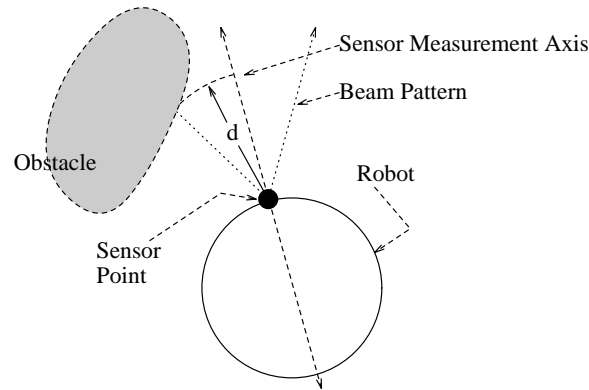
FIGURE 2.19. Centerline model.
