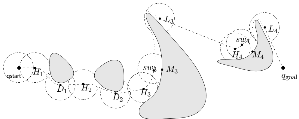
FIGURE 2.11. Path generated by Tangent Bug with finite sensor range. The dashed lines correspond to the motion - to - goal behavior and the dotted lines correspond to boundary-following. The dashed-dotted circles correspond to the sensor range of the robot.
