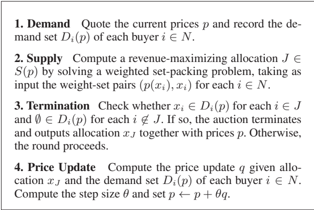
Figure 1: Generic auction round.
