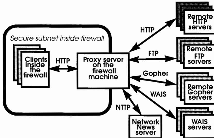
Figure 1. Overall setup of a proxy. Proxy server is running either on a firewall host or other internal host which has full internet access, or on a machine inside the firewall making connections to the outside world through SOCKS or other firewall software.
