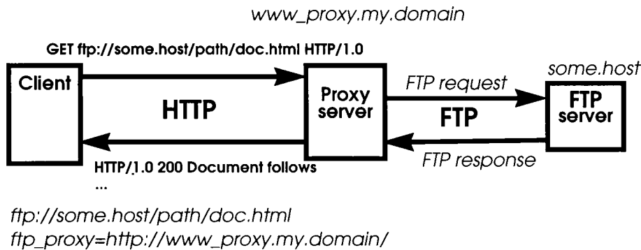
Figure 4. A proxied FTP transaction. Client makes a request to the proxy server, using HTTP, even though the actual resource is served by an FTP server. The proxy server sees from the full URL that an FTP connection should be made, and retrieves the file from the remote FTP server. Result is sent back to the client using HTTP.
