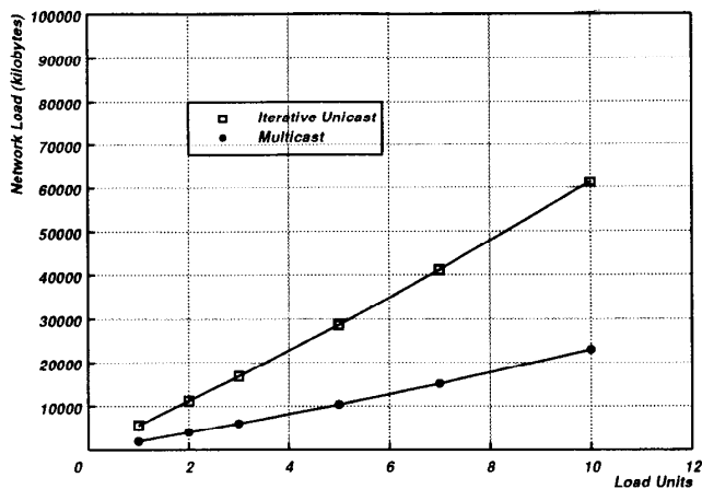
Fig. 4. Effect of Multicast on bytes transmitted.
