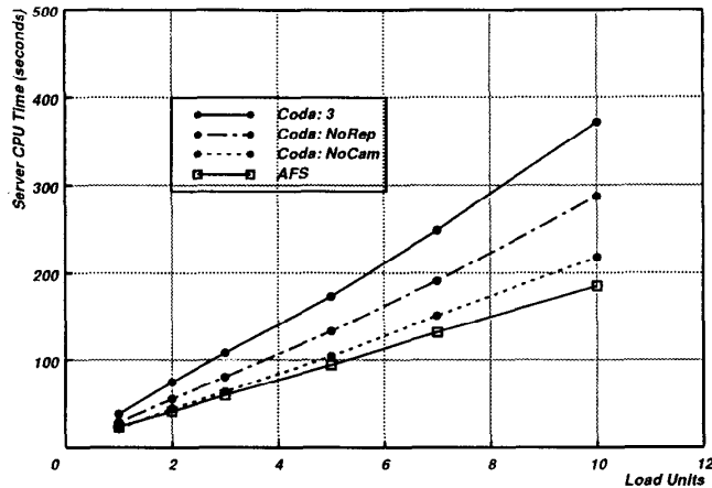
Fig. 3. Effect of load on server CPU utilization. This graph shows total number of server CPU seconds used as a function of load in running the benchmark. The configuration corresponding to the curve labeled "Coda:NoCam" is described in the text of Section VIII-C.
