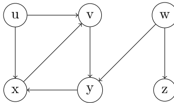
Figure 1: An example directed graph, G . A possible DFS of this graph would be (u \rightarrow v \rightarrow y \rightarrow x), (w \rightarrow z) . As we go as far as we can without before backtracking, we would not search an order such as (u \rightarrow v \rightarrow x) , as we would in some searching algorithms such as breadth-first search.
