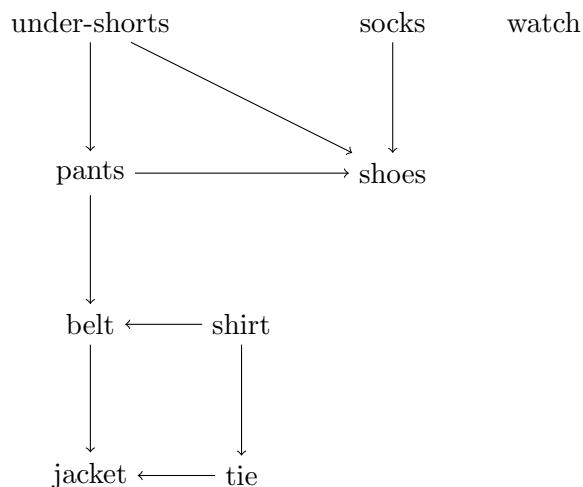
Figure 3: An example scenario (from [?] Section 22.4) involving topological sort. Consider the possible scenario of dependencies when getting dressed, shown in the figure by arrows, e.g., under-shorts must be put on before pants, and pants must be put on before shoes. A topological sort of this graph gives a valid ordering of putting on clothes that satisfies the dependencies. For example, (1) socks, (2) under-shorts, (3) pants, (4) shoes, (5) watch, (6) shirt, (7) belt, (8) tie, (9) jacket, would be a possible topological sort of the graph.
