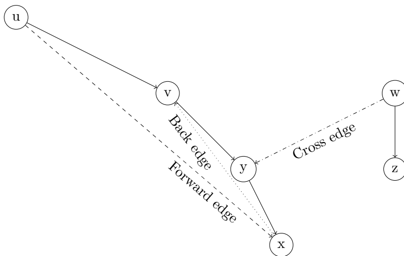
Figure 2: The DFS forest for the example search in figure 1. The edges in the forest are shown as solid lines — the dotted lines are other edges of the graph that are not part of the forest.
