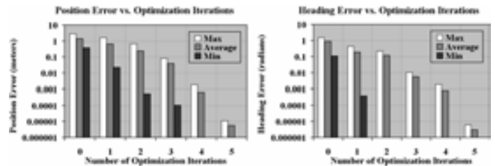
Figure 15: Trajectory Generator Convergence for Instrument Placement Tasks using All-Wheel Steering Mobility Systems. For the sequence of trajectories shown in Figure 14, the maximum, average, and minimum position and heading errors of the seven planned trajectories are shown as a function of the number of iterations executed by the trajectory generation algorithm.
