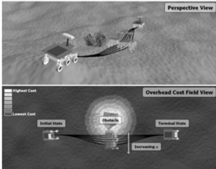
Figure 20: Minimizing Path Cost. The optimal control formulation of the trajectory generator can be used to minimize an arbitrary path cost function over the course of a trajectory. This example demonstrates avoidance of high cost regions (proximity to a simulated obstacle) at the expense of longer path lengths.
