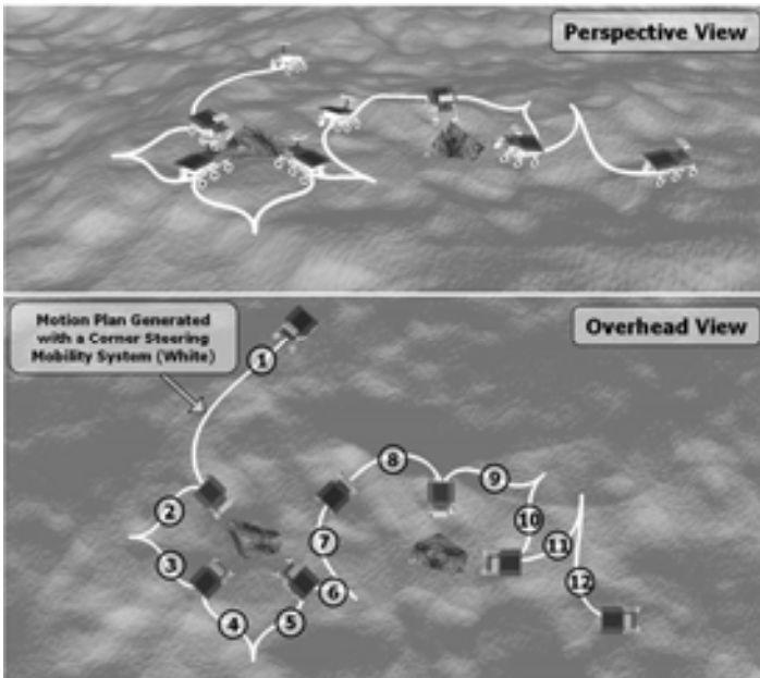
Figure 12: Instrument Placement using Corner Steering Mobility Systems. Sequences of trajectories are planned for an example instrument placement task using a corner steering mobility system. The targets must be aligned with the front of the robot chassis because of the location of the scientific instruments. Each of the seven science targets are achieved by planning twelve trajectories that include forward and backward motions.
