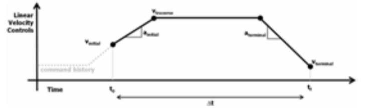
Figure 4: Trapezoidal Linear Velocity Profile. Typically most of the parameters defining the shape of the linear velocity control are known. For a trapezoidal velocity profile, the parameters in the control are the initial (v_0) , intermediate (v_{\text{traverse}}) , and terminal (v_f) velocities, initial (a_0) and terminal (a_f) accelerations, and the duration (\Delta t) .
