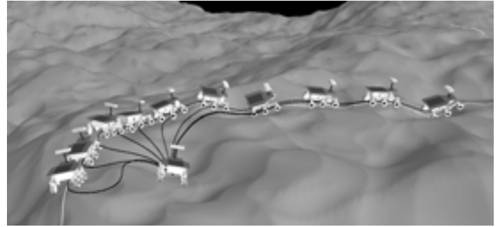
Figure 27: Reacquiring the Target Path. The rough terrain trajectory generation algorithm can be employed in a constrained optimization sense to determine the optimal corrective path to reacquire the target path. A cost function based on cross-track error, smoothness, and other factors is minimized in order to determine the optimal corrective trajectory.
