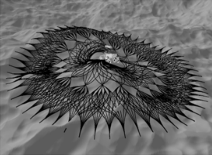
Figure 25: Terrain-Adaptive Ego-graphs. The ego-graphs generated in Figure 21 can be adapted to rough terrain using the developed trajectory generation algorithm in order to better evaluate dynamic feasibility and path cost. The fact that individual trajectories all pass exactly through the intended terminal states indicates compensation for terrain shape.
