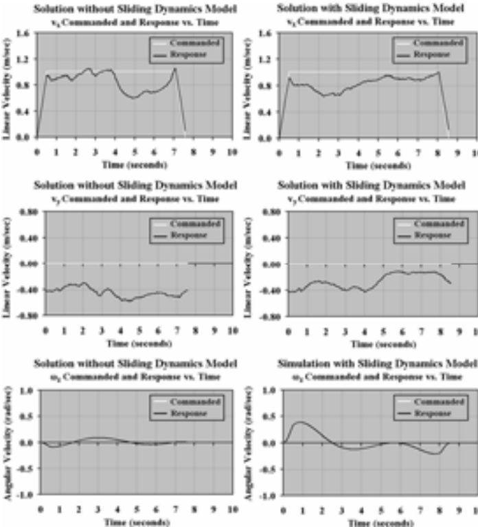
Figure 19: Compensating for Vehicle Sliding Dynamics in Trajectory Generation. Vehicle sliding dynamics models can be incorporated in the forward model of the vehicle to predictably compensate for these effects in trajectory generation.
