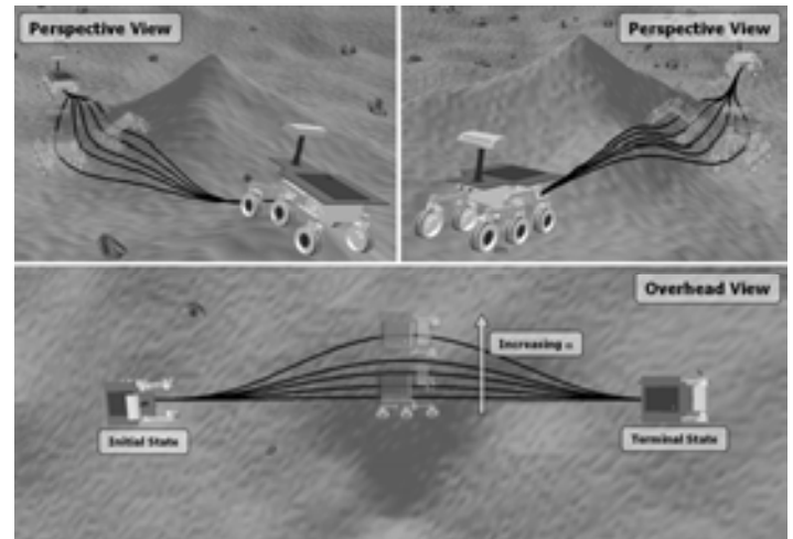
Figure 20: Minimizing Path Cost. The optimal control formulation of the trajectory generator can be used to minimize an arbitrary path cost function over the course of a trajectory. This example demonstrates avoidance of high cost regions (proximity to a simulated obstacle) at the expense of longer path lengths.
