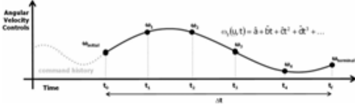
Figure 6: Spline Angular Velocity Profile. An alternate representation of a polynomial function is a spline function. The parameters in this control are the knot points ( \omega_1, \omega_2, \omega_3, \dots ) that define the shape of the angular velocity control and the duration ( \Delta t ). This representation is beneficial for numerical optimization schemes because all of the knot points have roughly equal scale.
