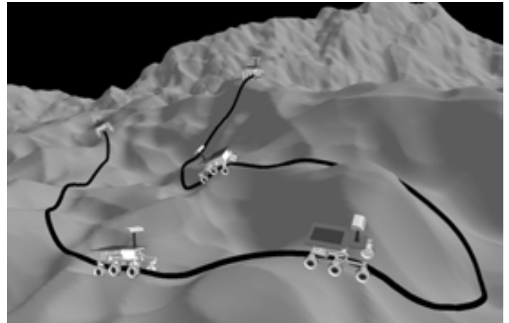
Figure 1: Motion Planning on Rough Terrain. For competent navigation in challenging environments, the terrain shape must be considered in the generation of continuous motion trajectories. The presented trajectory generation algorithm generates motion plans that account for arbitrary terrain shape, vehicle dynamics models, and wheel/terrain interaction models by linearizing and inverting forward models of propulsion, suspension, and motion.
