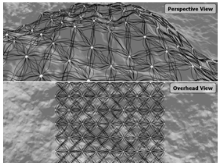
Figure 28: Connectivity of a State Space Lattice in Rough Terrain. The states of a lattice which is equally distributed in (x,y) can be connected with minimum-time paths in general rough terrain using our trajectory generator.
