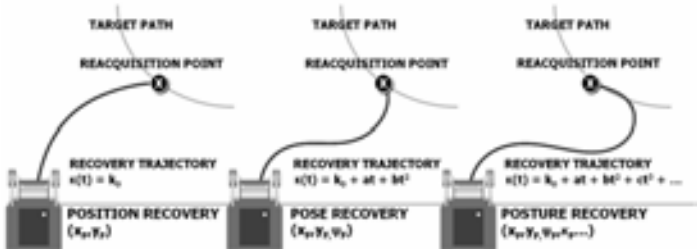
Figure 26: Corrective Trajectory Continuity. This figure demonstrates several different trajectory generation boundary conditions that lead to increasingly higher levels of continuity for corrective trajectories. The corrective trajectory becomes increasingly complicated at the benefit of higher degrees of terminal state continuity.
