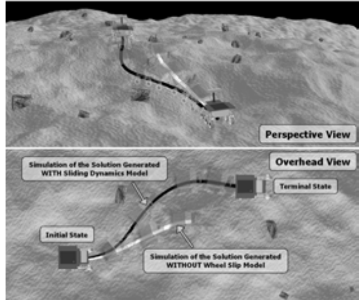
Figure 16: Compensating for Wheel Slip in Trajectory Generation.
