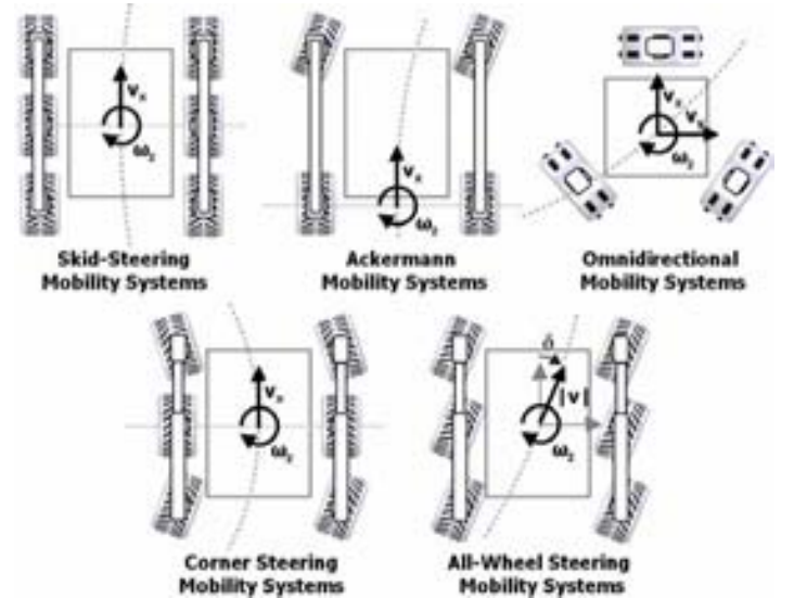
Figure 3: Mobility System Models. The choice of mobility system determines the vehicle's capacity to execute complex motions. Omnidirectional mobility systems are most capable, allowing instantaneous motion in any direction in the local tangent plane. All-wheel steering mobility systems allow motion in any direction in the local tangent plane, but are restricted by nonholonomic constraints. The skid-steering, Ackermann steering and corner steering mobility systems are the least flexible mobility systems because their linear velocity is constrained along the forward x-axis of the vehicle frame.
