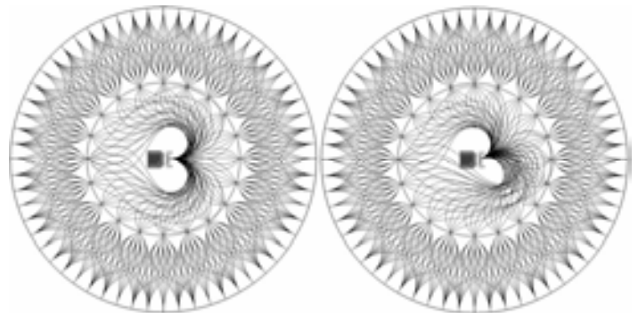
Figure 24: Ego-graph Generation. The presented trajectory generation algorithm can be used to generate ego-graphs, which are body-frame fixed obstacle avoidance and local navigation search spaces. The above two ego-graphs, comprised of 630 individual trajectories each, were generated with different initial states using the present algorithm. Note that only the first level of the search space is dependent on the current vehicle state.
