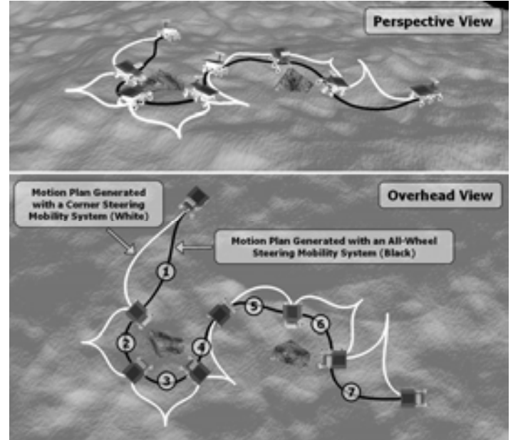
Figure 14: Instrument Placement using All-Wheel Steering Mobility Systems. The same instrument placement problem in Figure 12 is solved using an all-wheel steering mobility system, allowing the vehicle path heading to change independently from the body yaw. Each of the seven science targets are achieved by planning only seven motions. The overall motion plan (black path) is more efficient than the corner steering motion plan (white path) by effectively exploiting the all-wheel steering mobility.
