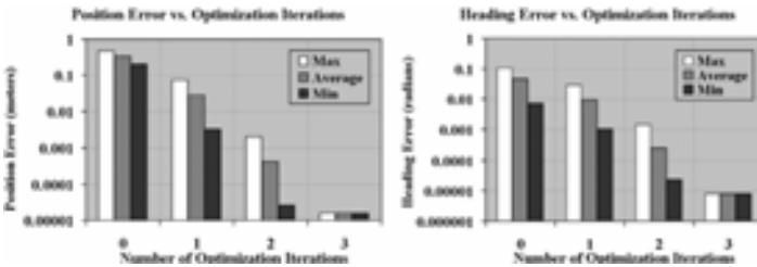
Figure 13: Trajectory Generator Convergence for Instrument Placement Tasks using Corner Steering Mobility Systems. For the sequence of trajectories shown in Figure 12, the maximum, average, and minimum position and heading errors of the twelve planned trajectories are shown as a function of the number of iterations executed by the trajectory generation algorithm.
