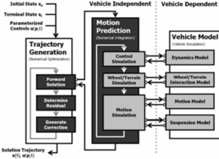
Figure 2: Trajectory Generator System Architecture. The trajectory generation algorithm can be conceptualized as a three-level hierarchy. The highest level is a numerical optimization that minimizes the constraint error by adjusting the free parameters in the controls. The next level, motion prediction, is simply the numerical integration of the equations of motion. The lowest level, the vehicle model, simulates the vehicle's dynamics, motion, and suspension. This architecture is formalized and implemented to permit different vehicle models to interface with the same underlying algorithm.
