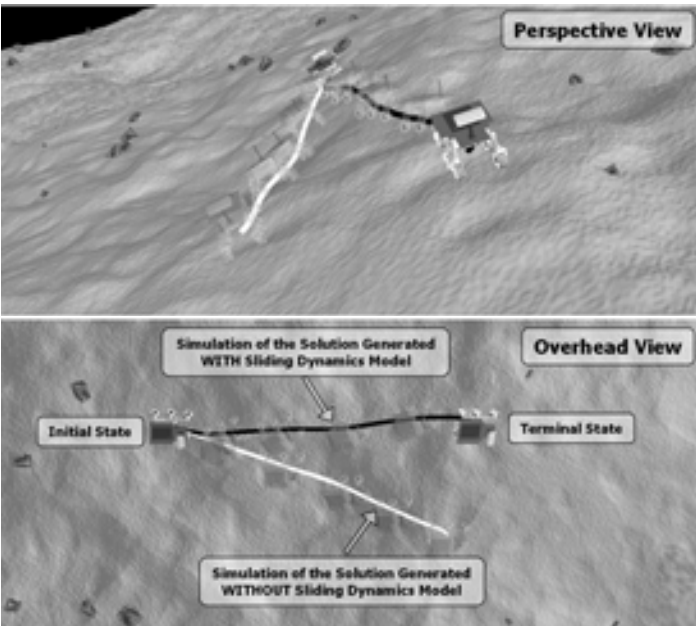
Figure 19: Compensating for Vehicle Sliding Dynamics in Trajectory Generation. Vehicle sliding dynamics models can be incorporated in the forward model of the vehicle to predictably compensate for these effects in trajectory generation.
