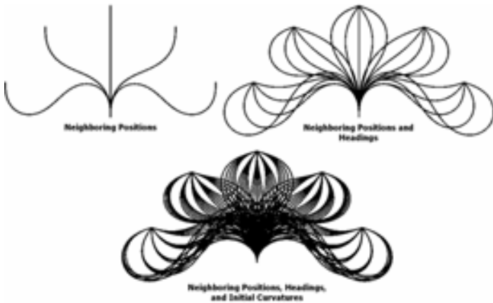
Figure 7: Neighboring Solutions for Initial Guess Lookup Table Generation. The initial guess lookup table is generated by continually solving neighboring trajectory generation problems in such a way that the last solution is a good initial guess for the next query.
