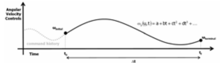
Figure 5: Polynomial Angular Velocity Profile. A polynomial function of time is an effective parameterization of the angular velocity controls. The parameters in the control are the polynomial coefficients (a, b, c, \dots) and the duration (\Delta t) .
