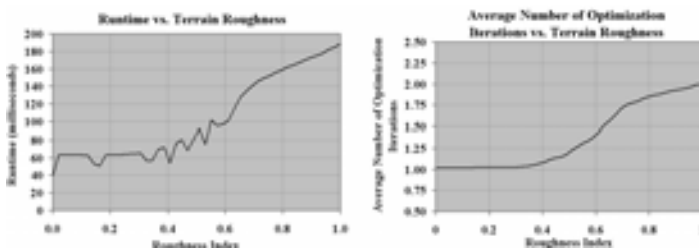
Figure 22: Terrain Roughness Tests. In order to conduct a fair series of runtime vs. terrain roughness tests, motions plans are generated on a series of terrains of increasing roughness ranging from a roughness index of 0.0 (nominally flat terrain) to 1.0 (very rough terrain).
