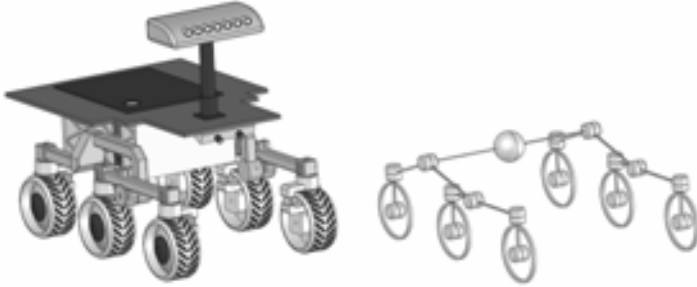
Figure 8: Kinematic Models for Rocky 8. A kinematic model can easily be generated for mobile robots with Rocker-Bogie suspensions using a series of revolute joints. The kinematic model is used to map body frame velocities to wheel frame velocities and to determine the attitude and elevation of the robot given its position.
