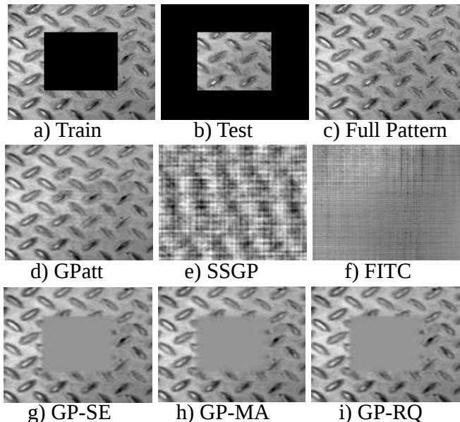
Figure 1. Extrapolation on a Metal Tread Plate Pattern. Missing data are shown in black. a) Training region (12675 points), b) Testing region (4225 points), c) Full tread plate pattern, d) GPatt-30, e) SSGP with 500 basis functions, f) FITC with 500 pseudo inputs, and the SMP-30 kernel, and GPs with the fast exact inference in Section 4.1, and g) squared exponential (SE), h) Matérn (MA), and i) rational quadratic (RQ) kernels.
