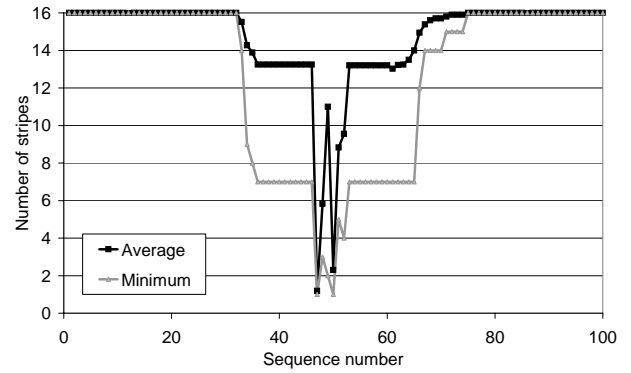
Figure 19: Number of stripes received versus sequence number.
