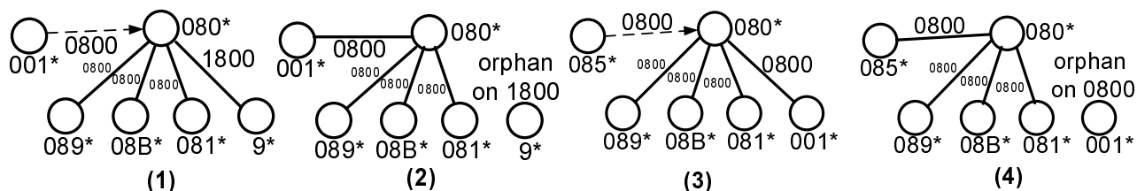
Figure 5: Handling of prospective children by a node that has reached its outdegree limit. Circles represent nodes and the numbers close to them are their nodeIds (* is a wildcard). Solid lines indicate that the bottom node is a child of the top node and the number close to the line is the stripeId. Dashed lines represent requests to join a stripe. The node with id 080* has reached its outdegree limit of 4. (1) Node 001* requests to join stripe 0800. (2) Node 080* takes 001* as a child and drops 9*, which was a child in stripe 1800 that does not share the first digit with 080*. (3) Then node 085* requests to join stripe 0800. (4) Node 080* takes 085* as a child and drops 001*, which has a shorter prefix match with stripe 0800 than other children.
