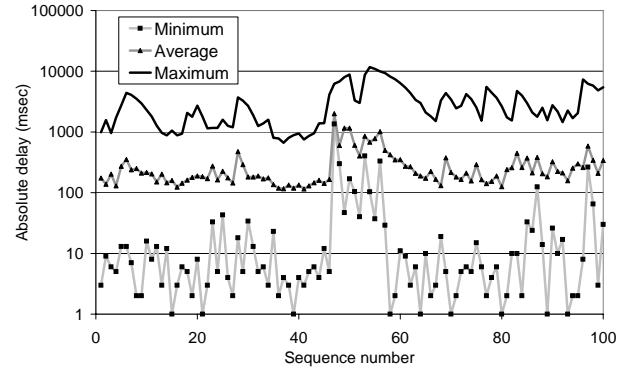
Figure 20: Packet delays versus sequence number.
