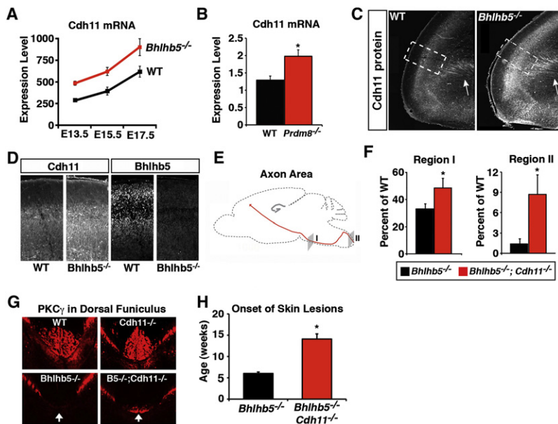
Figure 7. Cdh11 Is a Key Target of the Bhlhb5/Prdm8 Repressor Complex
