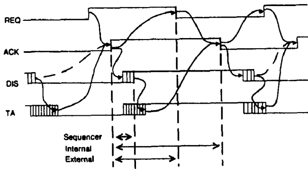
Figure 3-3: Synchronizer timing
