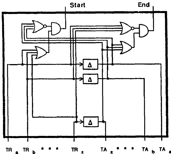
Figure 4-1: The controller for path P
