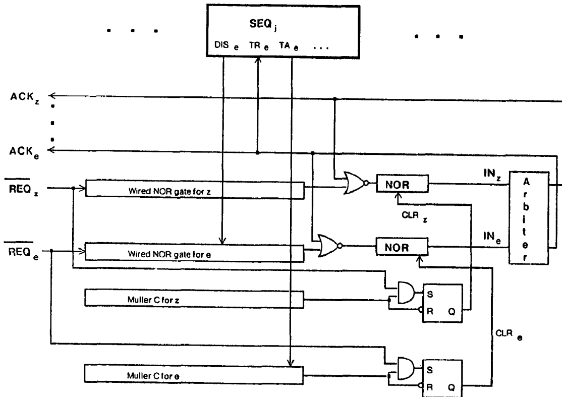
Figure 3-2: A synchronizer circuit
