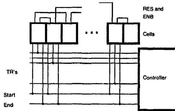
Figure 4-7: The floorplan for a sequencer
