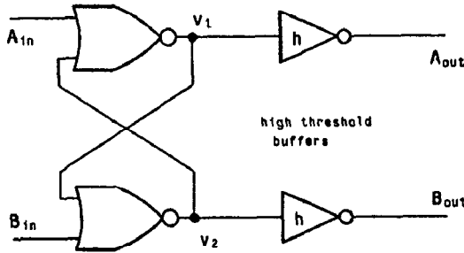
Figure 5-2: Seitz's Interlock Element
