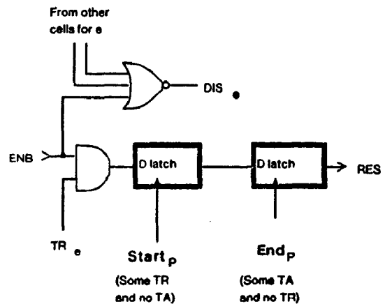
Figure 4-2: Cell for event e in path P
