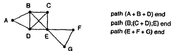
Figure 5-1: The conflict graph of a path expression
