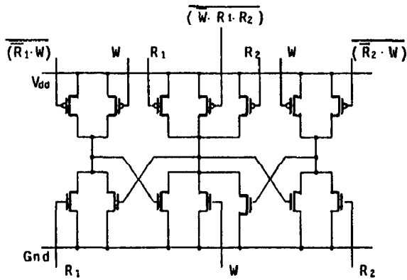
Figure 5-4: The Arbiter for 1-Writer-2-Readers Problem in CMOS.
