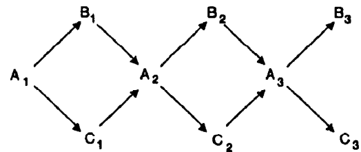
Figure 2-1: An example pomset
