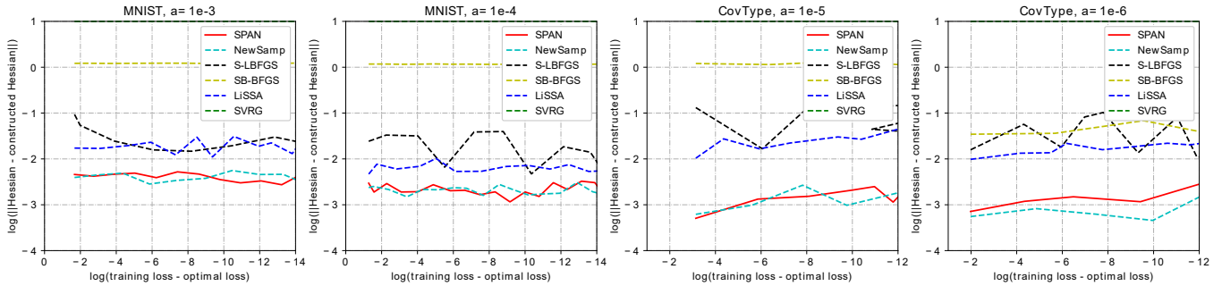
Figure 3: Hessian approximation error. Notice that SPAN achieves near lowest error.
