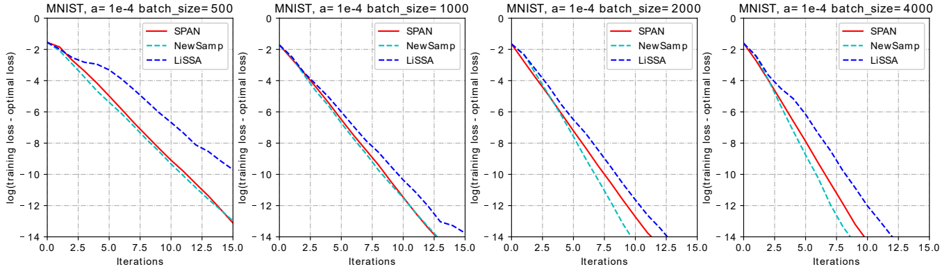
Figure 4: Empirical convergence rate comparison on MNIST4-9 dataset. Four columns represent different batch-size for sub-sampled Hessian.
