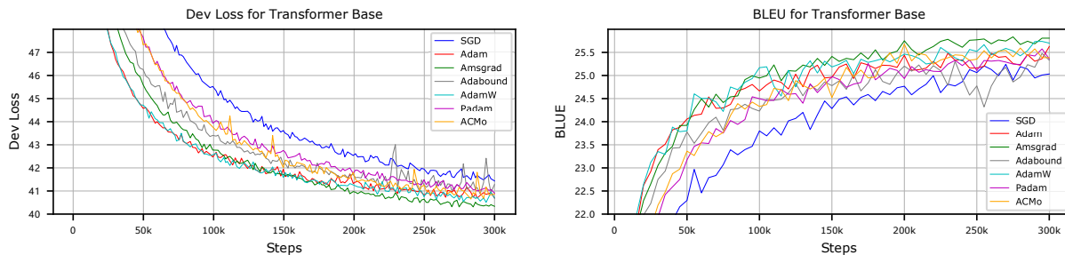
Figure 4: Learning curves of optimizers for Transformer-base on WMT'14 EN-DE machine translation task. (Dev loss & BLEU score)
