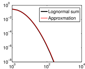
Fig. 3. Lognormal sum
