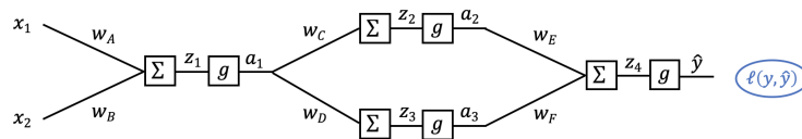
Figure 5: Neural Network
