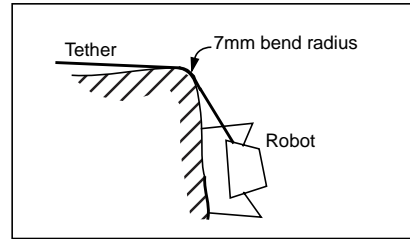
Fig. 3. Severe tether loading condition
