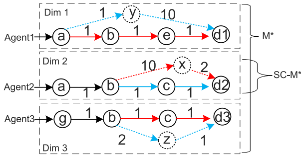
Fig. 2. Example of applying M* and SC-M* to an MAPP problem with three agents. Solid vertexes and arrows denote individually optimal paths. Dotted vertexes and arrows are the nodes and edges added during expansion. Blue and red arrows are specific edges picked by M* and SC-M*, respectively. Black arrows are common edges picked by both algorithms. Traditional M* has to expand all three dimensions due to hard-collision constraints while SC-M* considers soft-collision constraints and only expands dimension 2.
