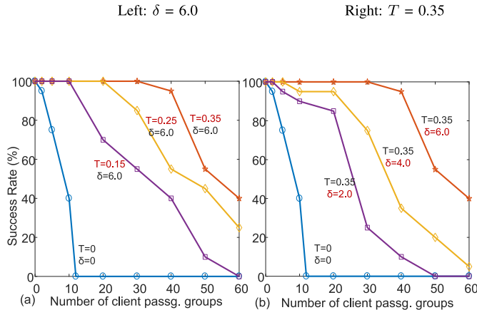
Fig. 10. (a) The impact of the collision threshold T on the success rate of SC-M*, given \delta = 6.0 ; (b) The impact of the offset parameter \delta on the success rate, given T = 0.35 .
