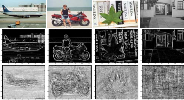
Fig. 2. In top to bottom form, each image is followed by its gradient and reconstructed image structure from top 150 eigenvectors. Categories are airplane, motorcycle, leaf and background.
