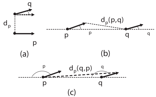
Figure 2. Distances in different cases: (a) flow vectors p and q are on parallel curves; (b,c) p and q are on the same curve, and q follows p . (b) shows the distance D(p, q) where (c) shows the distance D(q, p) .
