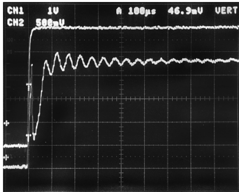
Figure 18. Typical Turn-On Response at V_{DD} = 5 \text{ V}
