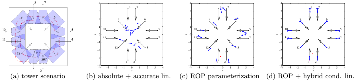
Figure 3: The performance of the Kalman Filter on a simulated network of cameras. The long arrows indicate the true location and orientation of the cameras, the ellipses (often small) are 95% confidence intervals in the position estimates, and the two short arrows (often overlapping) are the 95% confidence intervals in the estimate of orientation. (a) Eight side-facing and four overhead cameras are placed around a hallway. The dark-shaded regions represent the overlapping fields of the view. The dotted line shows the location of the object at each time step. (b) Nonlinearities give poor results when camera poses are represented as (x, y, \theta) , even with accurate linearization of the observations. (c) The ROP representation of camera poses improves results. (d) Combining ROP with the hybrid conditional linearization techniques gives excellent results.
