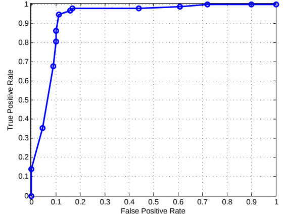
Fig. 6. ROC curve for the HMM-based classifier.
