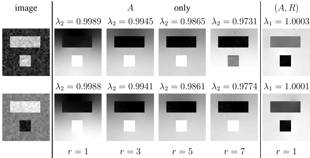
Figure 3.6: Repulsion can bind multiple objects with less computation. We use \sigma_1 = 0.1 to evaluate affinity by intensity, 3% of which become negative with \beta = 5 . Column #2-5: results with attraction measured by G(x; \sigma_1) with increasing r 's. Column #6: result with affinity measured by h(x; \sigma_1, 5\sigma_1) . Row #1: the image has two rectangles of equal average intensity 0.8 against background of 0.5, added by Gaussian noise with standard deviation 0.03. A much larger neighborhood size is needed for attraction to achieve a comparable result with repulsion. Row #2: the smaller object now has an average intensity of 0.2. Even with a large r , the two objects cannot be united by attraction.
