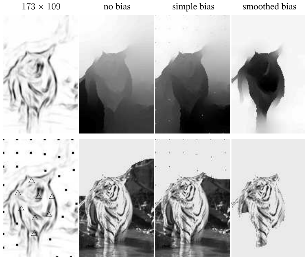
Figure 5.6: Segmentation with partial grouping from brightness. Column #1: edge magnitudes and biased nodes (29 pixels marked as \blacksquare , 8 pixels marked \triangle ) having extreme intensities. Columns #2-4: the second eigenvector and foreground images obtained with no constraints, simple constraints U and smoothed constraints P^T U respectively.
