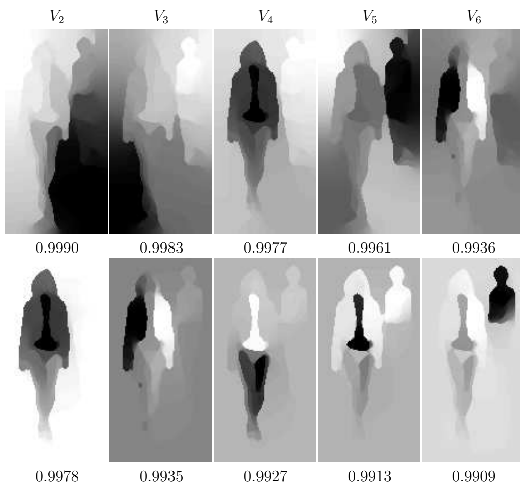
Figure 5.8: Segmentation with partial grouping from spatial attention. Image size: 180 \times 90 . Row #1-2: leading eigenvectors of unconstrained and constrained normalized cuts respectively. Uniform V_1 's are omitted. Numbers are eigenvalues. It takes 27.2 and 19.7 seconds respectively to compute these eigenvectors in MATLAB on a PC with 1GHz CPU and 1GB memory.
