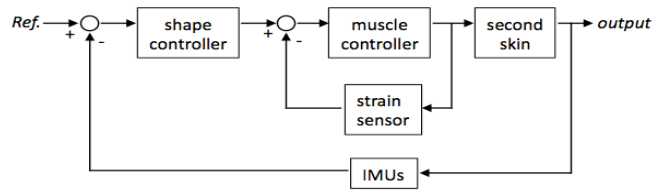
Fig. 7 Block diagram for controlling Second Skin
