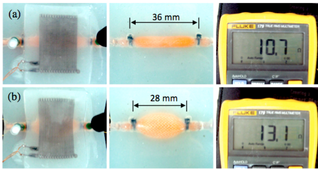
Fig. 2 Sensor-actuator unit embedded in a silicone elastomer. (a) Relaxed artificial muscle. (b) Contracted artificial muscle. (Front side with strain sensor, backside without strain sensor, and sensor resistance, respectively.)
