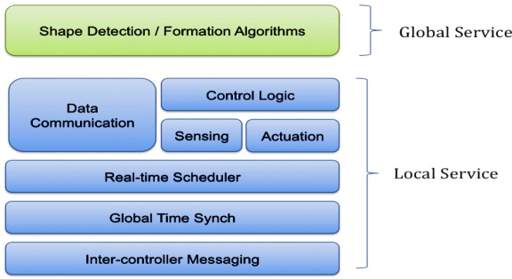
Fig. 8 Second Skin controller platform software architecture.
