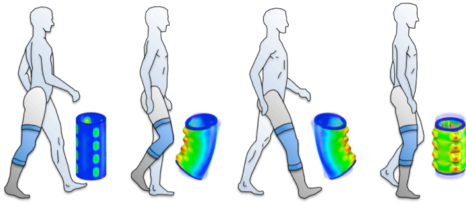
Fig. 11 Possible shape changes of Second Skin during gait cycle: relax for toe-off, bending for midswing, opposite bending for heel strike, and stiffening for midstance, respectively.
