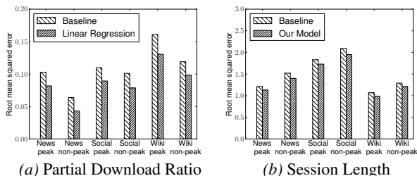
Figure 15: Our models are more accurate than the baseline in predicting partial download ratio.
