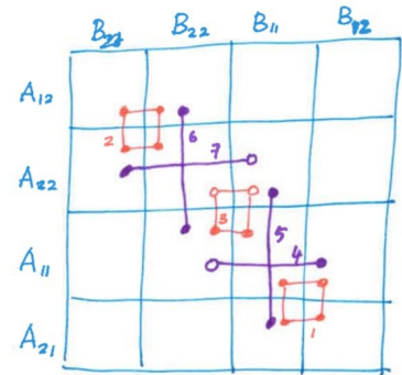
Figure 1.2: Strassen's Multiplications.
