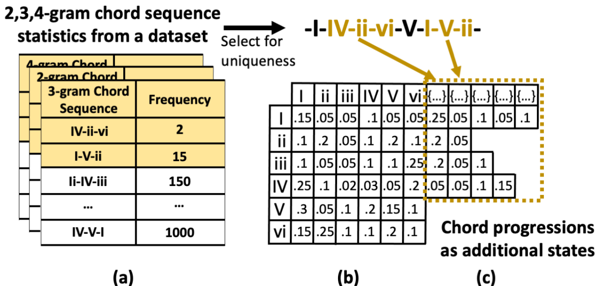
Figure 5: Distinctive chord sequence detection.
