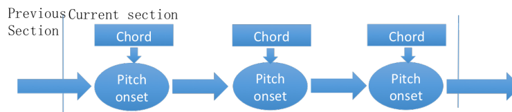
Figure 7: Pattern-based bass generation model using current chord for context and transition matrix for note-to-note probabilities.
