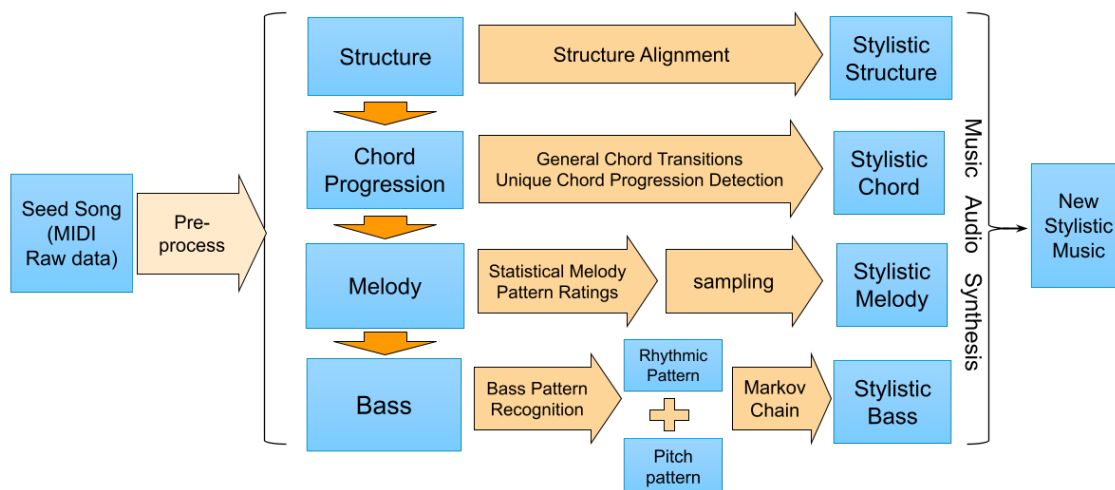
Figure 3: Framework of stylistic music generation system.
