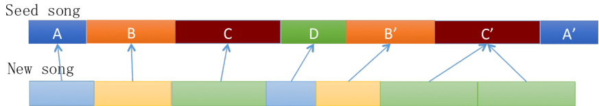
Figure 4: An example of ideal structure alignment.
