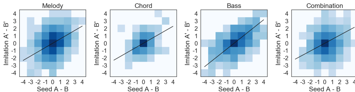
Figure 12: Correlation between preference-of-A – preference-of-B and preference-of-A’ – preference-of-B’ (all four values from the same listener), where A and B are seed songs, A’ and B’ are imitations.
