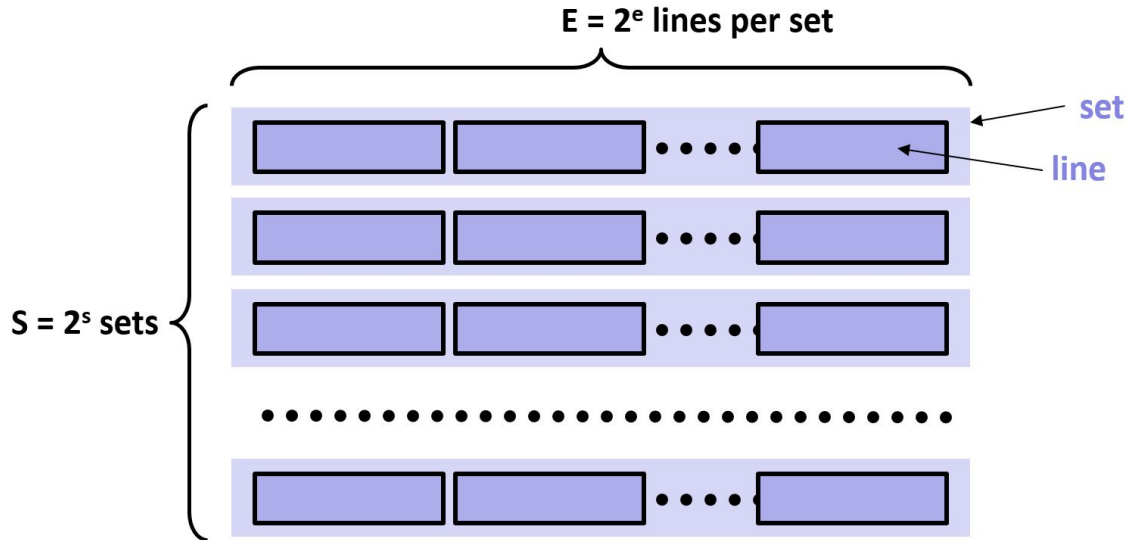
Figure 1: Cache
