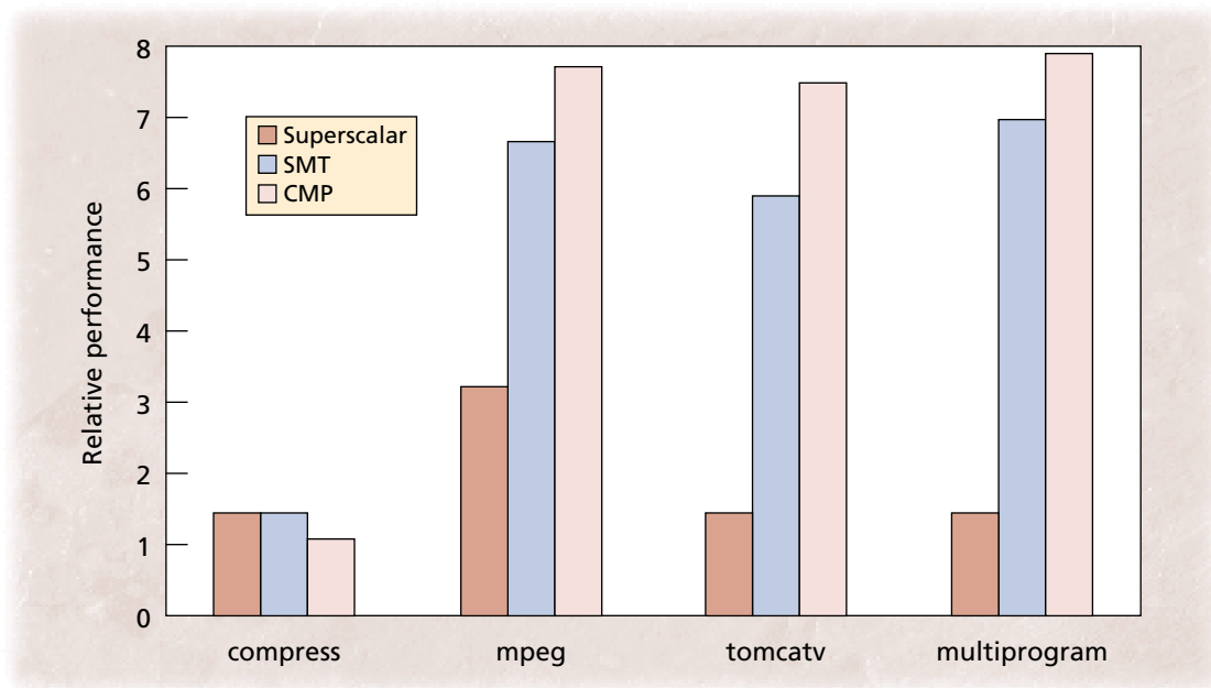
Figure 2. Relative performance of superscalar, simultaneous multithreading, and chip multiprocessor architectures compared to a baseline, 2-issue superscalar architecture.
