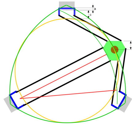
Bird's Eye view of a delta printer's range of motion from reprap.org
