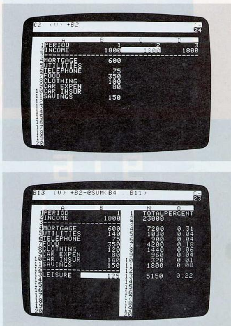
Figure 2. This simple Visicalc program display (top) shows four columns and 20 rows of home budget information. The cursor, an inverse video light bar controlled by key presses, is in position C2. The top command line shows that C2 is a value (as opposed to a text string) that has been set up to have the same value as position B2.
