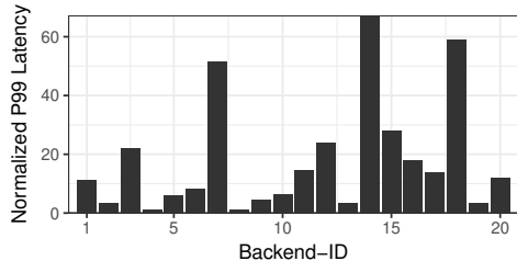
Figure 5: Normalized P99 latencies for the 20 most queried backends in the OneRF system during a typical 10 minute period. The backends are ordered by their query rates during this period. We see that query rate is not correlated with backend tail latency.
