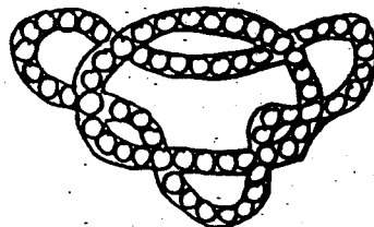
Figure 15. Hungarian Rings with multiple crossings
