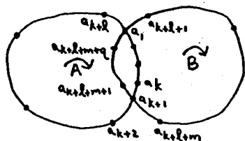
Figure 14. The Hungarian Rings
