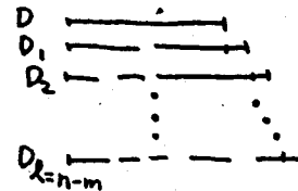
Figure 16. A tower of conjugates
