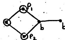
Figure 10. Swapping two pebbles
