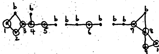
Figure 5. The subpuzzle starting positions
