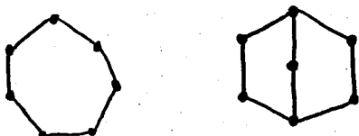
Figure 6. A Polygon; graph T_0
