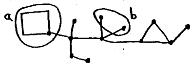
Figure 9. a: Biconnected leaf; b: "Multiple leaves"
