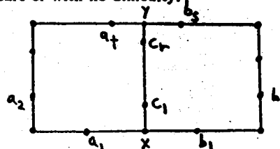
Figure 11. A T_2 -graph
