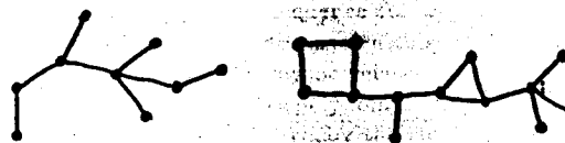
Figure 7. A Tree; a tree-like structure
